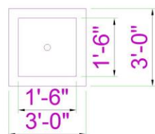
FOUNDATION PLAN
