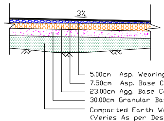
SECTION B-B PAVEMENT DETAIL FOR SERVICE ROAD
