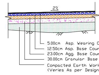
SECTION A-A PAVEMENT DETAIL FOR MAIN CARRIAGEWAY
