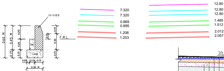
DETAIL OF KERB STONE
